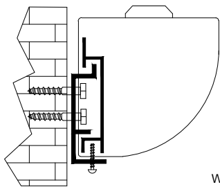
Mounting Diagrams
