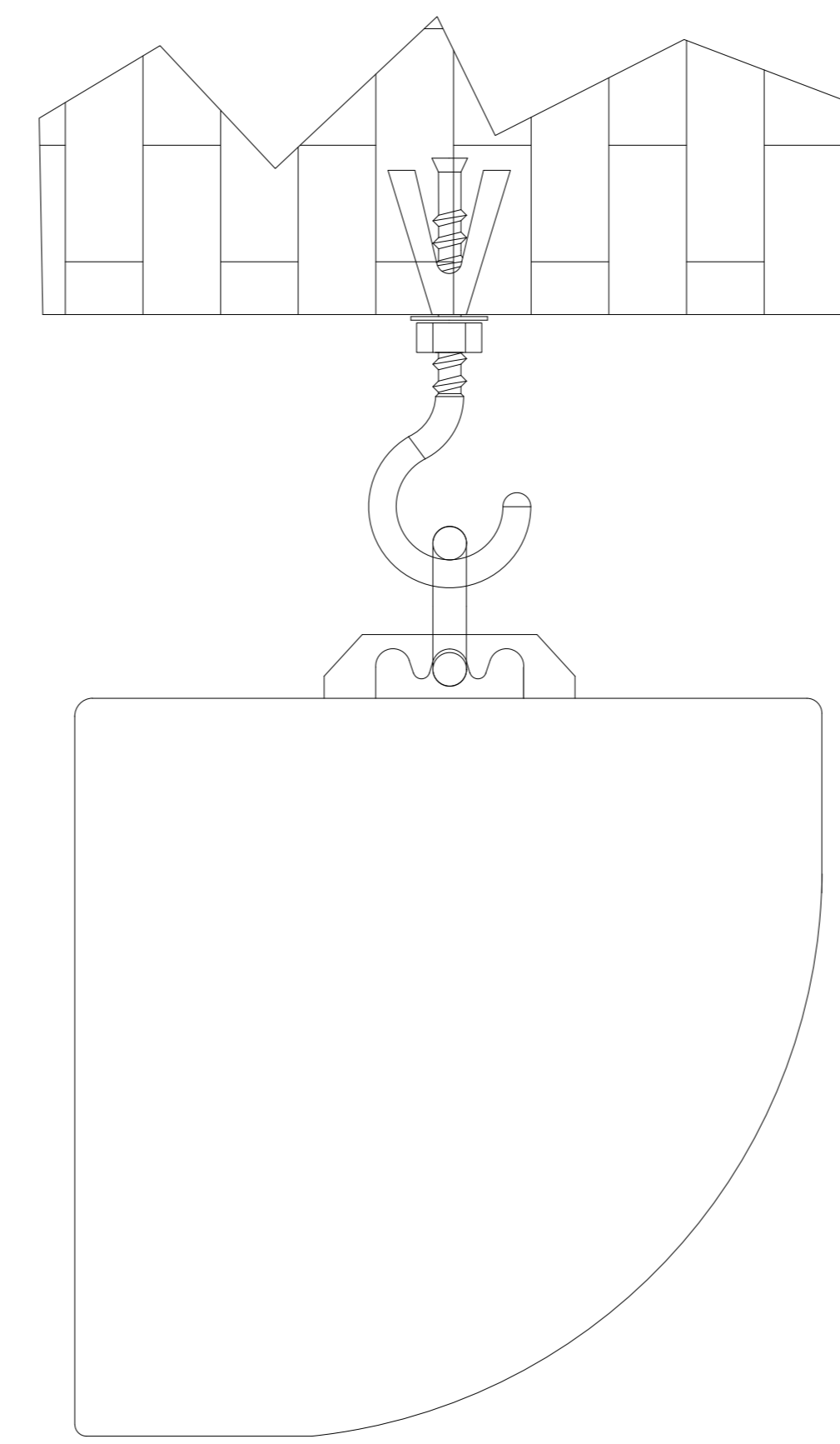
Ceiling Mounting
