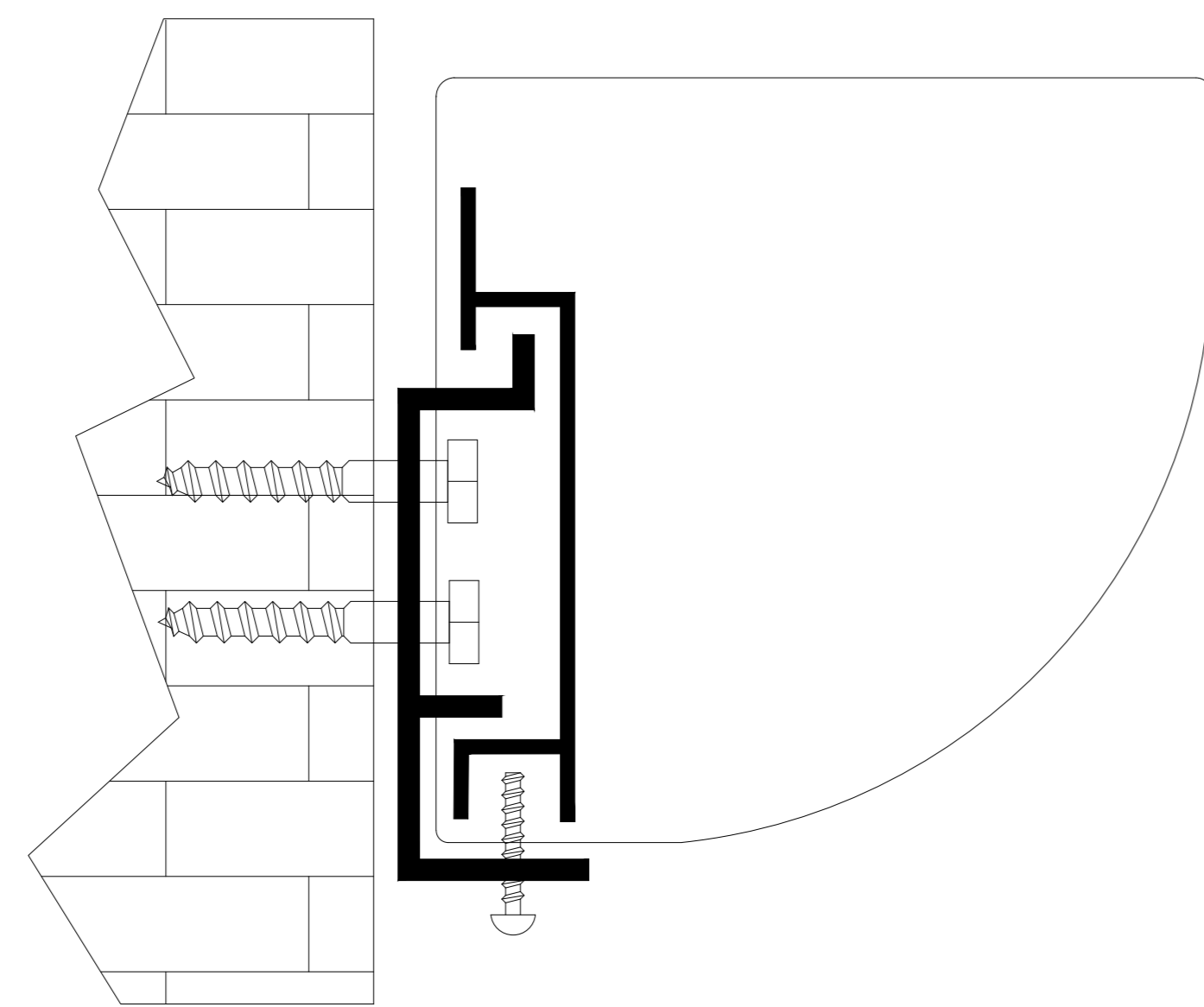
Wall Mounting
