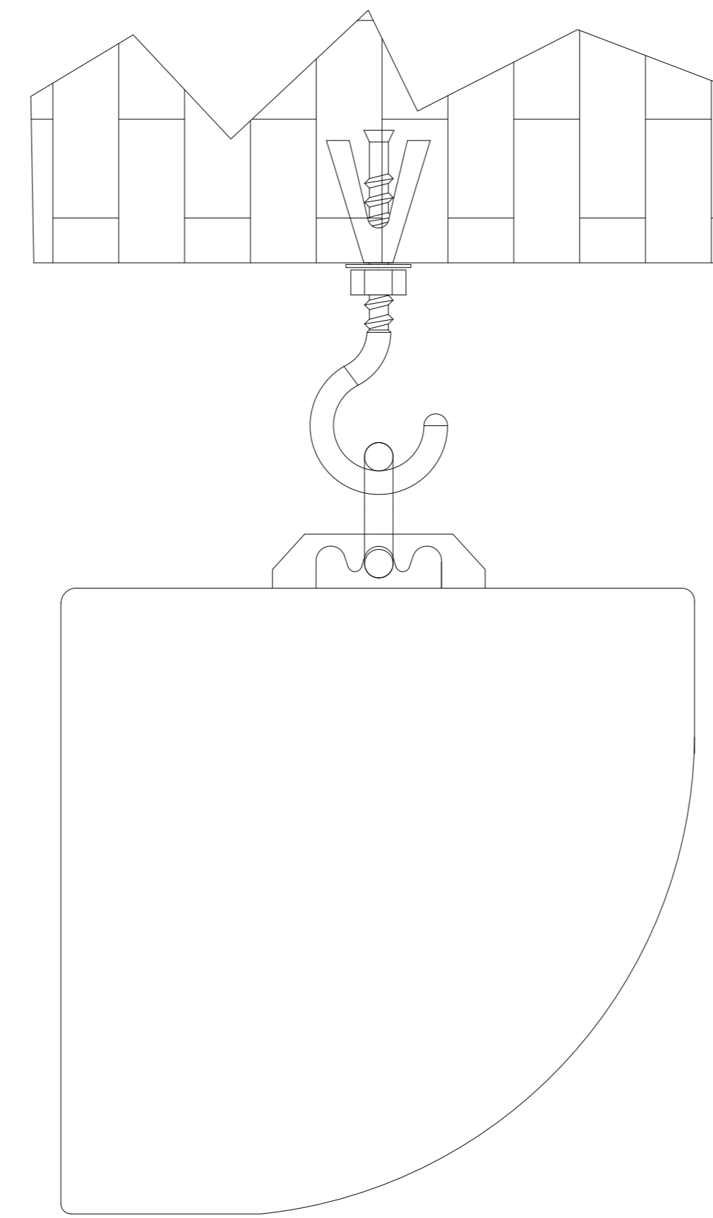
Ceiling Mounting
